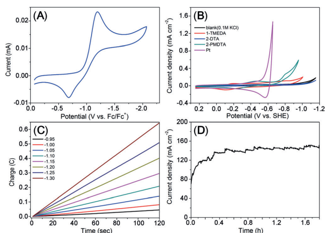
Figure 1. A) Cyclic voltammogram of 2 mM solution of 2-PMDTA in \text{CH}_3\text{CN} with 0.1 M of [n\text{Bu}_4\text{N}][\text{PF}_6] electrolyte. Scan rate: 50\text{ mVs}^{-1} . B) Cyclic voltammograms of blank (black), 1 mM aqueous solution of 1-TMEDA (red), 2-DTA (blue), 2-PMDTA (dark green) and Pt (magenta) with 0.1 M of KCl electrolyte. Scan rate: 50\text{ mVs}^{-1} . C) Charge consumption by the aqueous solution of 1 mM DNIC 2-PMDTA and 1 M KCl vs. time at different applying potentials (vs. SHE). D) Current density for the electrolysis of 1 mM DNIC 2-PMDTA in 1 M \text{KCl}_{(\text{aq})} at an applied potential of -1.2 V (vs SHE).
